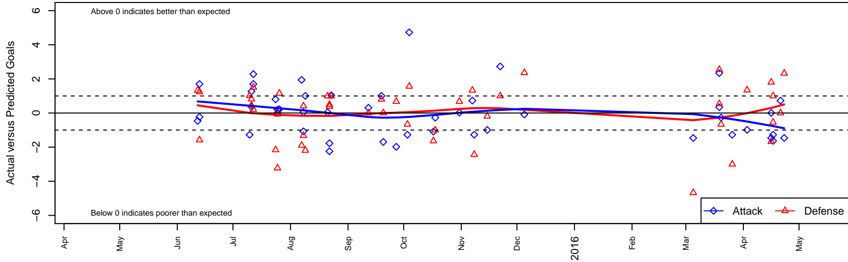
FC Edmonds Elite G01 Dots are actual minus expected GF (blue circles) and GA (red triangles). Blue line is smoothed change in attack strength. Red is smoothed change in defense strength.
